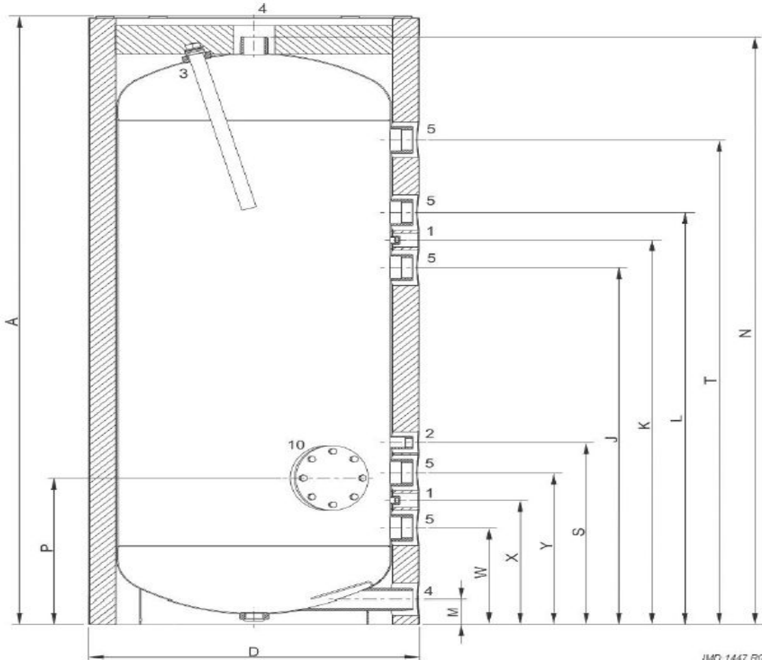
Dimensioned Sketch
