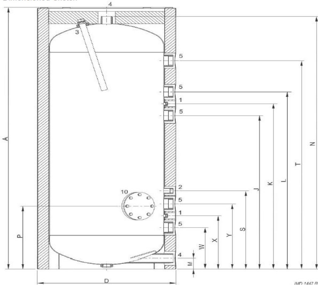
Dimensioned Sketch
