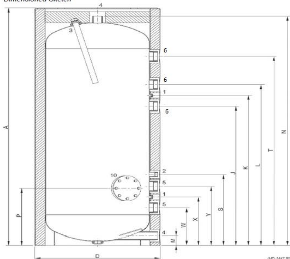
Dimensioned Sketch
