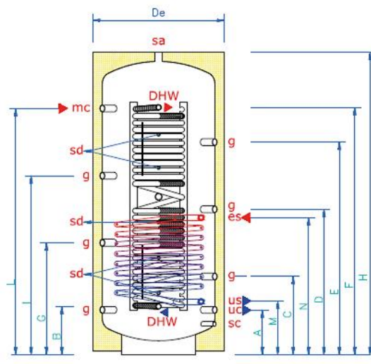
4.1.2 VERSION 2 DHW COIL AND SOLAR COIL
