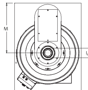
Concentric flue top view LBF120 to 240GCE
